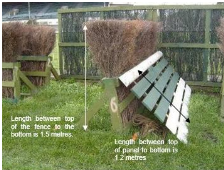
Removable Steeplechase Fence – Side Aspect
